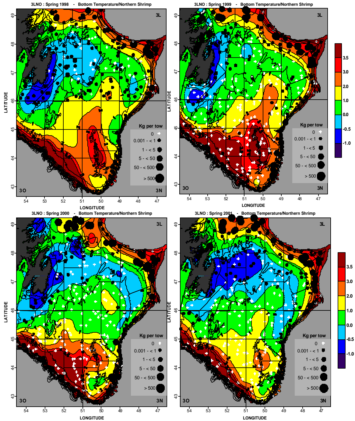
Fig. 5b. Bottom temperature contour maps (in ^{\circ}\text{C} ) for the spring of 1998-2001 from the annual Div. 3LNO survey. The total weight of shrimp in each fishing set is shown as solid circles. The white crosses represent zero catches.
