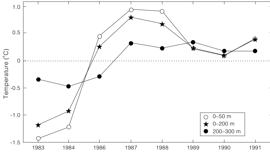
Fig. 6. Annual variation of temperature at the Cape Farewell section Station 4.
