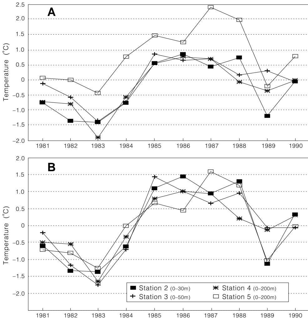
Fig. 7. Annual variation of temperature along the Fylla Bank section (A) based on mean 1963-91, (B) based on mean 1981-90 (0-30 m - Station 2; 0-50 m - Station 3; 0-200 m - Station 4, 5).
