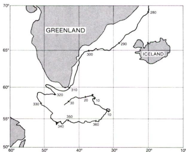
Fig. 8. Monitored track of an ice float from October 1984 (day 280) to February 1985 (day 35). (Courtesy of A. Clarke, Bedford Institute of Oceanography, Dartmouth, Nova Scotia, Canada).
