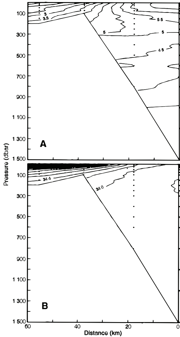
Fig. 4. Mean vertical distribution of (A) temperature ( ^{\circ}\text{C} ) and (B) salinity along the Discord section.
