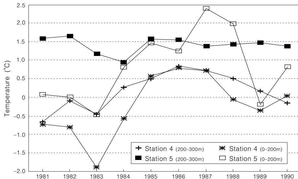
Fig. 9. Annual variability of temperature at Stations 4 and 5 of the Fylla Bank section with reference to the Irminger layer (200–300 m).
