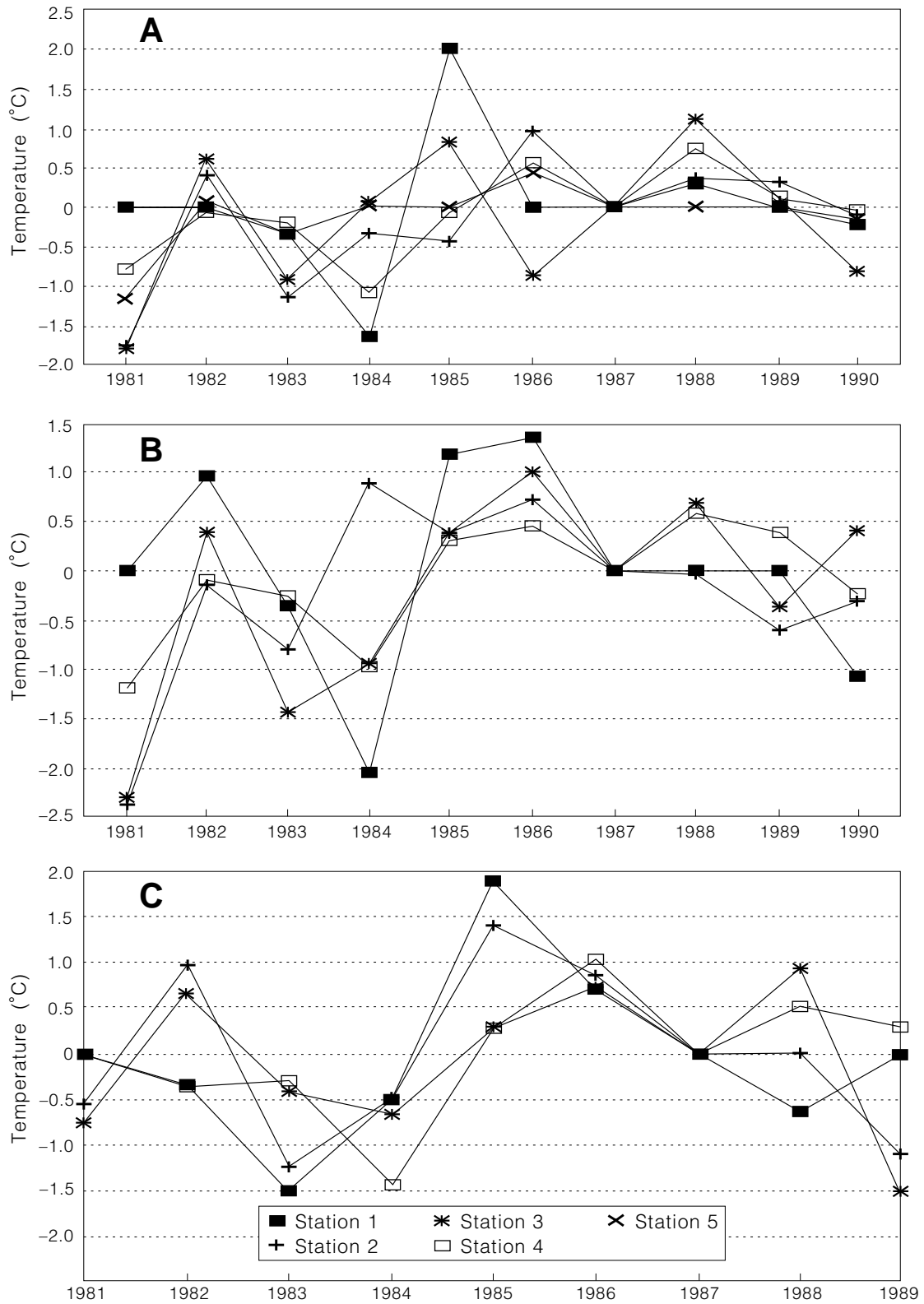
Fig. 5. Annual variation of temperature (0-200 m) along the (A) Mösting section, (B) Bille section and (C) Discord section.
