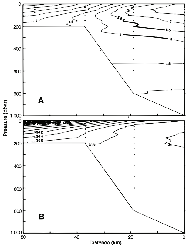
Fig. 3. Mean vertical distribution of (A) temperature and (B) salinity along the Bille section.
