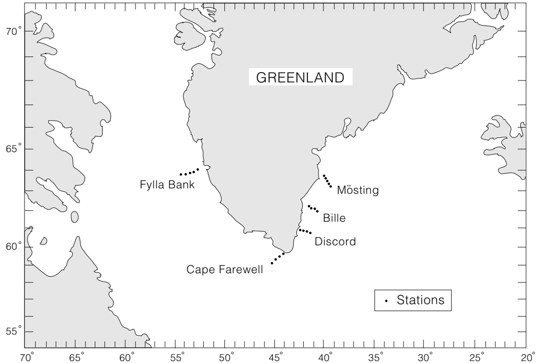
Fig. 1. Locations of sections and stations.
