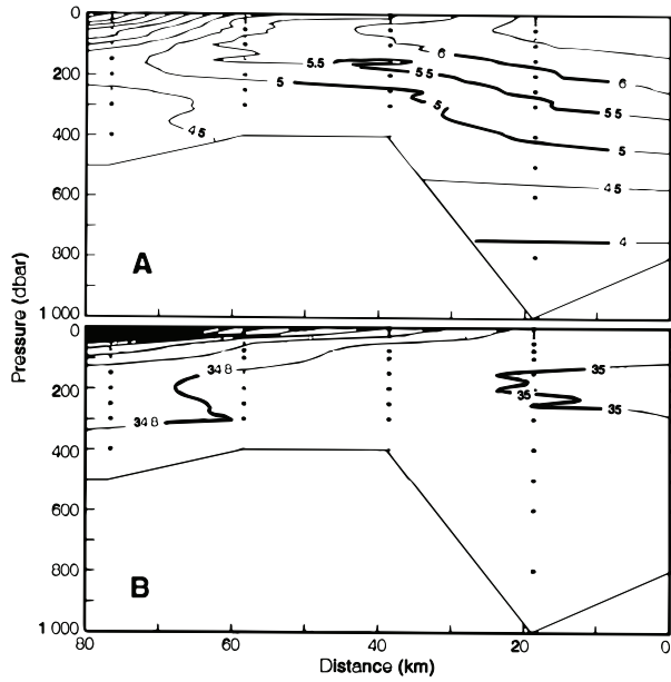
Fig. 2. Mean vertical distribution of (A) temperature ( ^{\circ}\text{C} ) and (B) salinity along the Mösting section.
