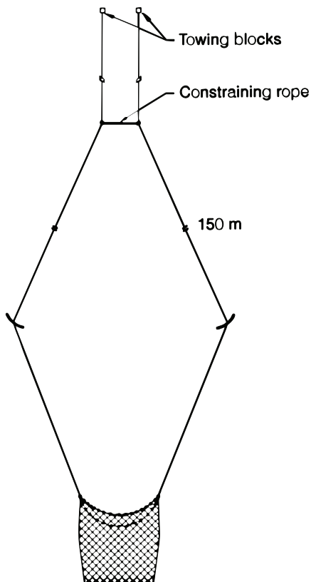
Fig. 13. Controlling trawl door spread using a rope strung 150 m ahead of the trawl doors. (Adopted from Engås and Ona 1993).
