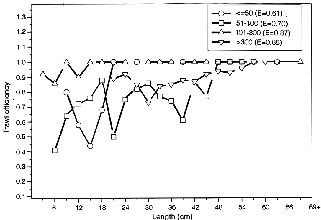
Fig. 12. Effect of density on trawl efficiency of cod derived from bag trawl escapement experiments. (Walsh and McCallum, unpublished data).
