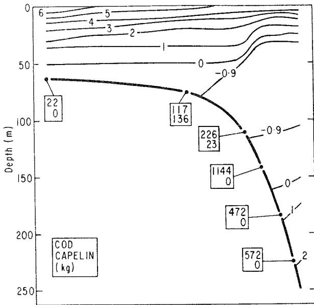
Fig. 2. Catches of cod and capelin in relation to temperature and depth at line R (see Fig. 1) on the eastern Grand Bank in June 1967.
