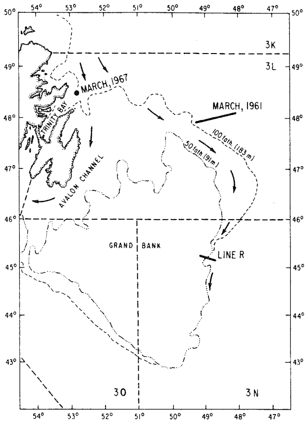
Fig. 1. Sampling positions and other locations mentioned in the text. Arrows indicate the general direction of Labrador Current flow.
