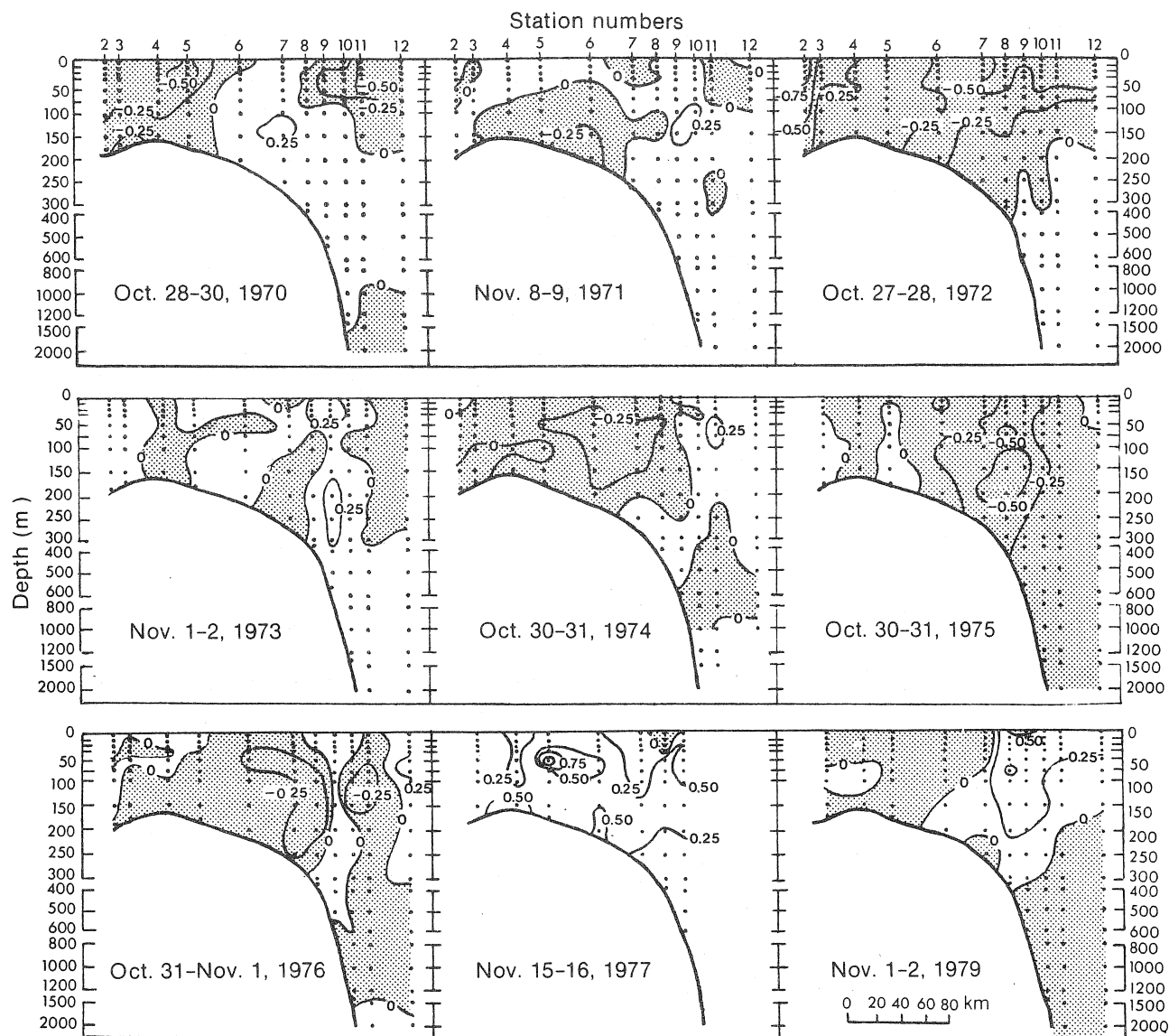
Fig. 6. Distribution of salinity anomalies for the Hamilton Bank section in October–November 1970–77 and 1979. (Zones of negative anomalies are shaded.)
