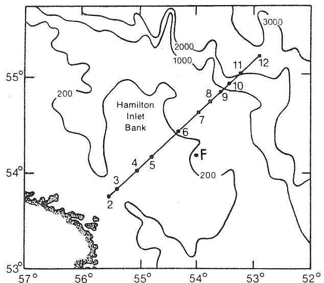
Fig. 1. Locations of oceanographic stations on USSR Section 8-A across Hamilton Bank off southern Labrador occupied during mid-October to mid-November in 1962, 1964–77, and 1979–80 (mean date, 31 October).
