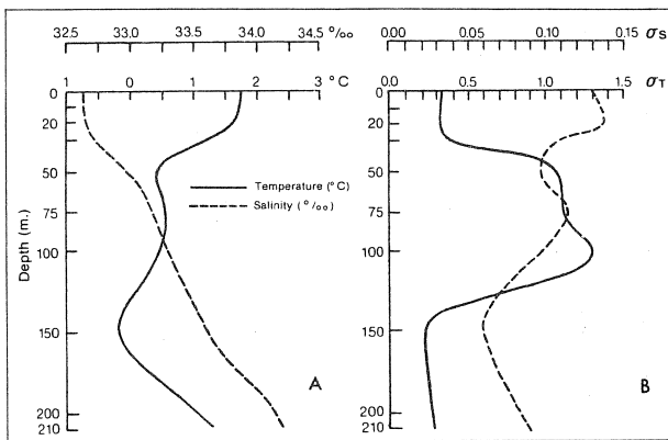
Fig. 7. Vertical profiles of average temperature and salinity (A) and corresponding standard deviations (B) at station F over a 24-hr period on 5–6 October 1980.
