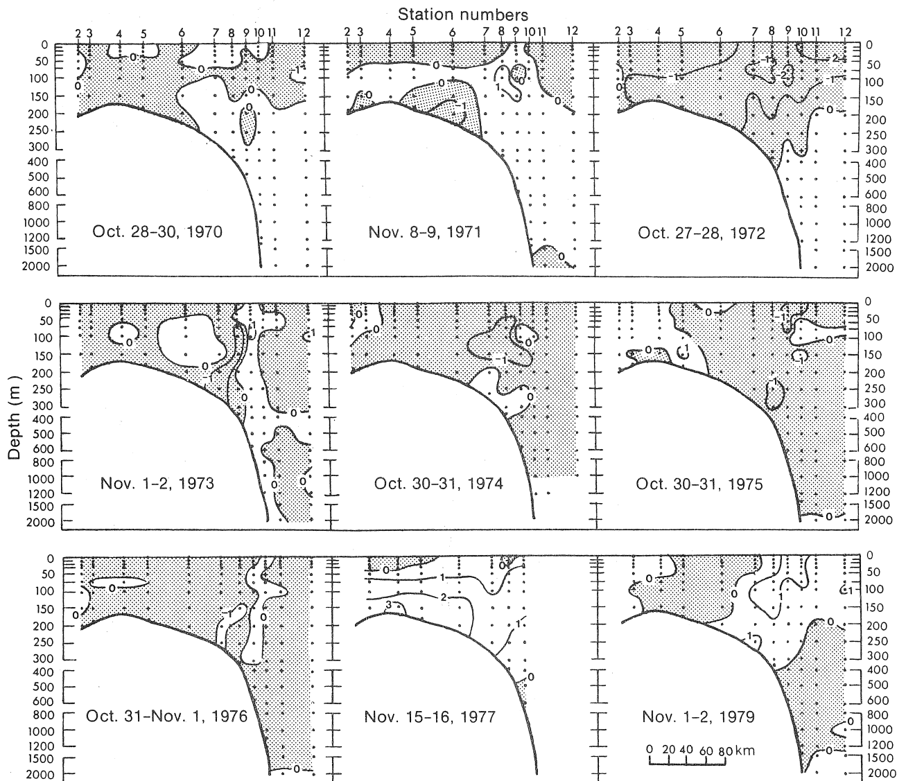
Fig. 5. Distribution of temperature anomalies for the Hamilton Bank section in October–November 1970–77 and 1979. (Zones of negative anomalies are shaded.)
