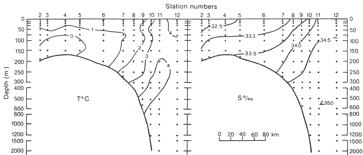
Fig. 2. Distribution of long-term mean temperature and mean salinity for the Hamilton Bank section shown in Fig. 1.
