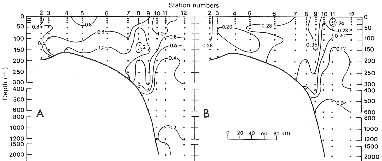
Fig. 4. Distribution of standard deviations of temperature (A) and salinity (B) from long-term mean values, for the Hamilton Bank section shown in Fig. 1.
