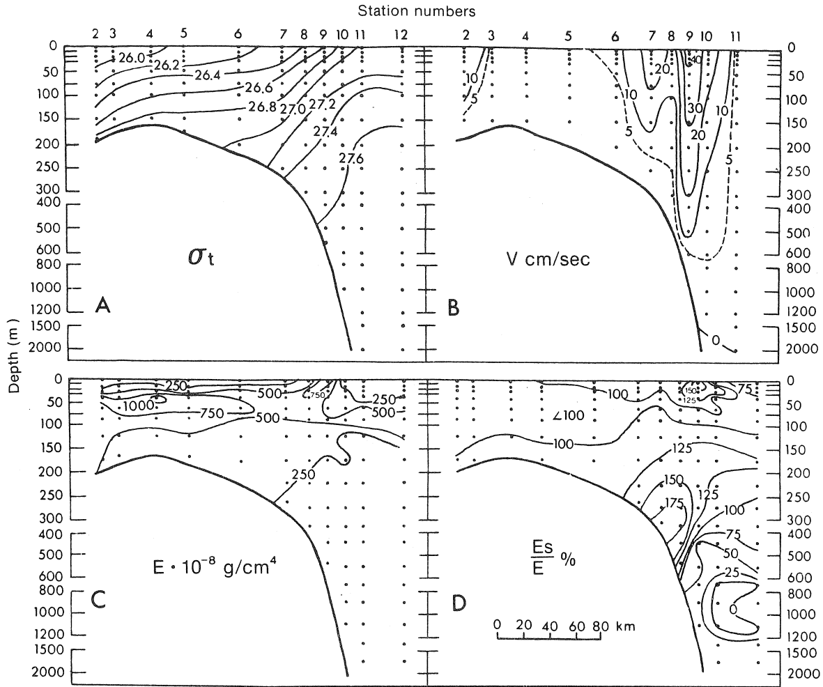
Fig. 3. Distribution of long-term mean density (A), velocity of geostrophic currents (B), stability of water layers (C), and contribution of salinity to stability (D), for the Hamilton Bank section shown in Fig. 1.
